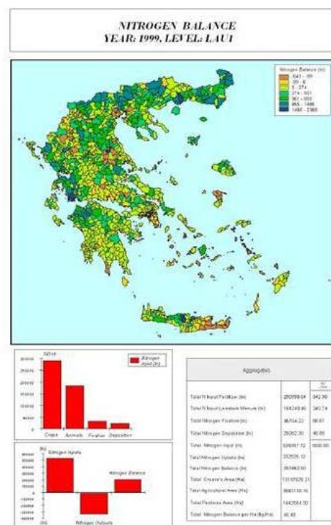
Figure 6. Nitrogen balance .
